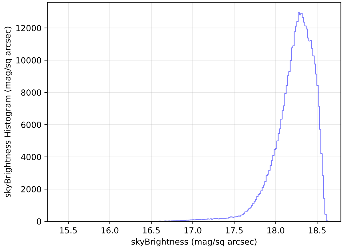
internal_u_expt27_nscale1.1v3.4_10yrs WFD y band: skyBrightness Histogram
