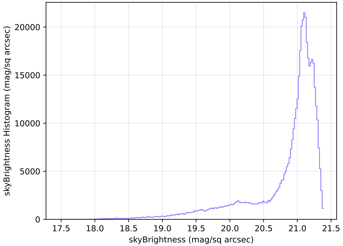
internal_u_expt27_nscale1.1v3.4_10yrs WFD r band: skyBrightness Histogram
