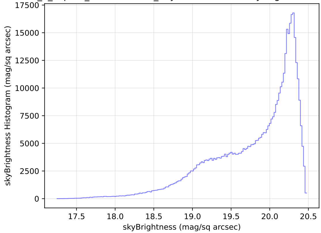
internal_u_expt27_nscale1.1v3.4_10yrs WFD i band: skyBrightness Histogram
