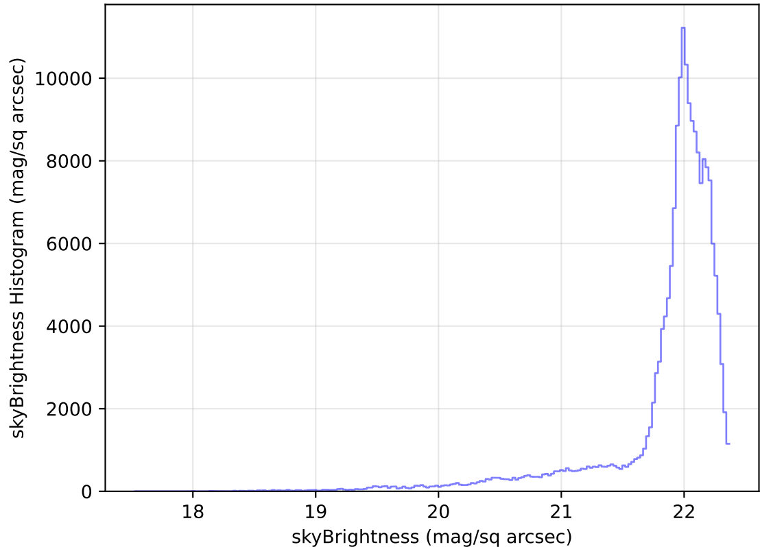
internal_u_expt27_nscale1.1v3.4_10yrs WFD g band: skyBrightness Histogram
