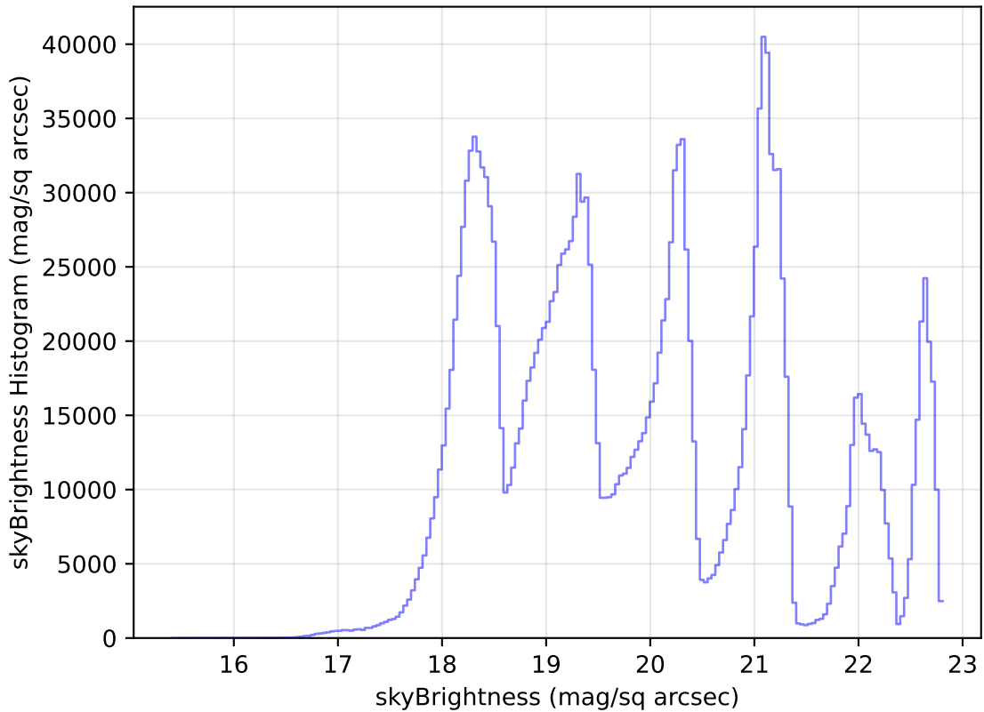
internal_u_expt27_nscale1.1v3.4_10yrs WFD all bands: skyBrightness Histogram
