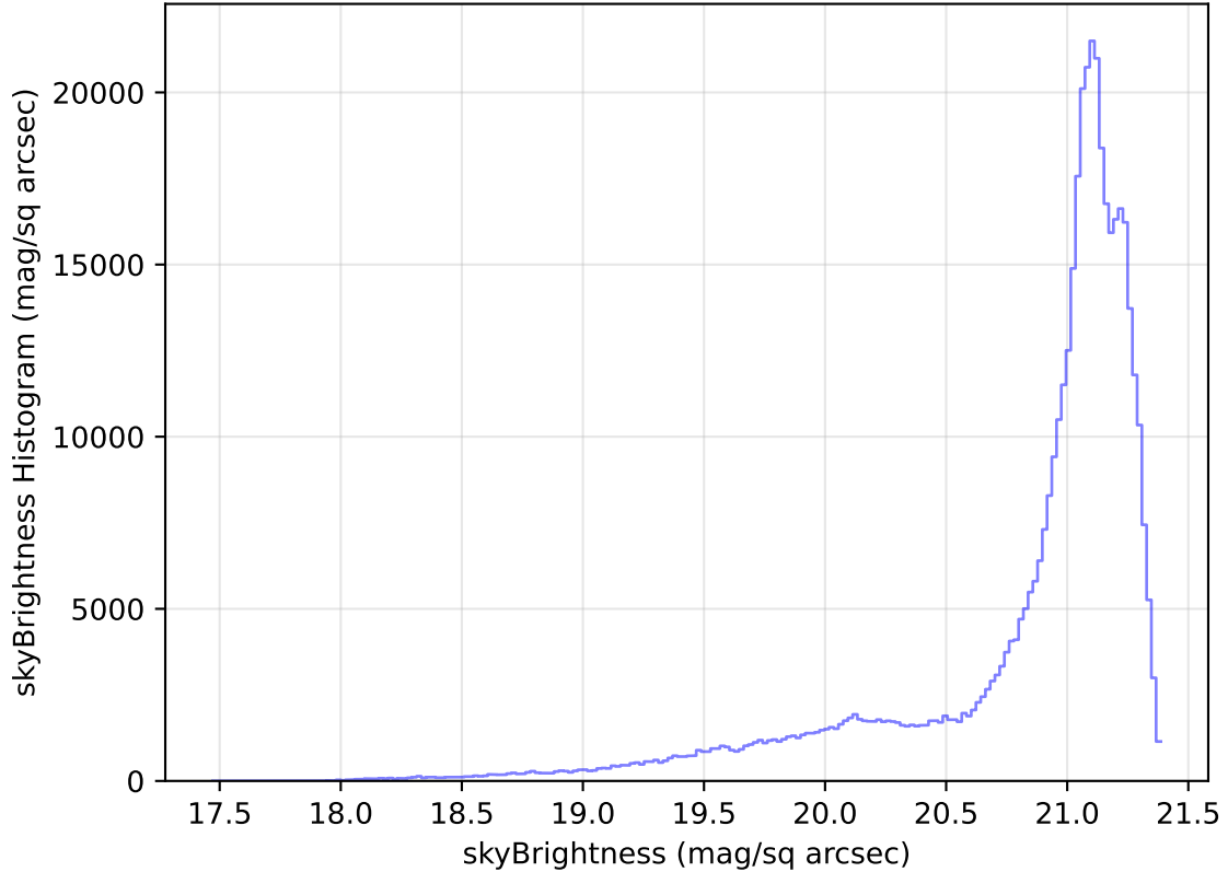
internal_u_expt27_nscale1.1v3.4_10yrs All sky r band: skyBrightness Histogram
