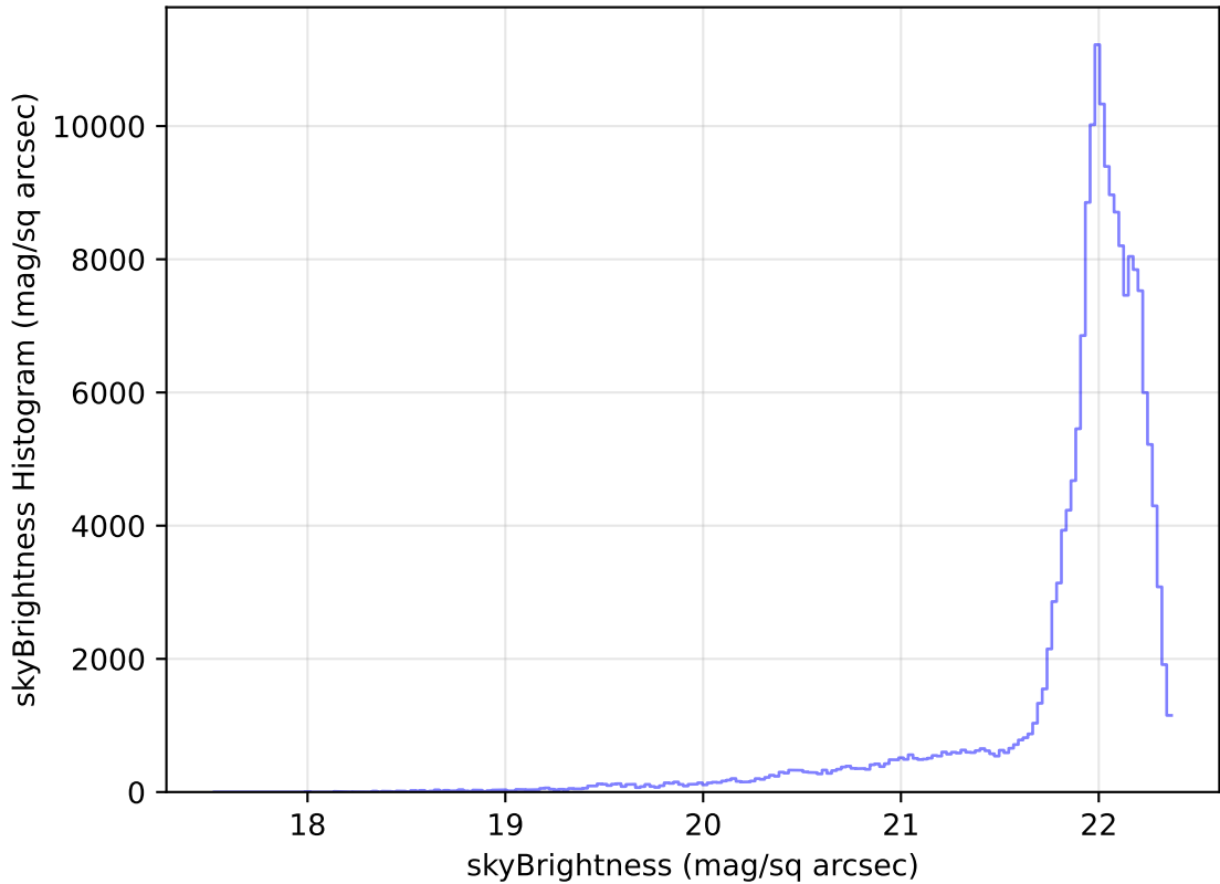
internal_u_expt27_nscale1.1v3.4_10yrs All sky g band: skyBrightness Histogram
