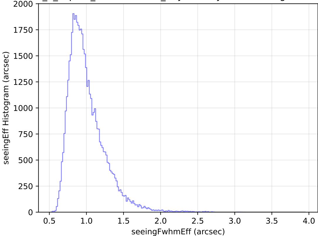
internal_u_expt27_nscale1.1v3.4_10yrs Yr 1 y band: seeingEff Histogram
