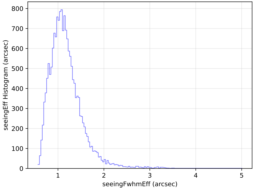
internal_u_expt27_nscale1.1v3.4_10yrs Yr 1 u band: seeingEff Histogram
