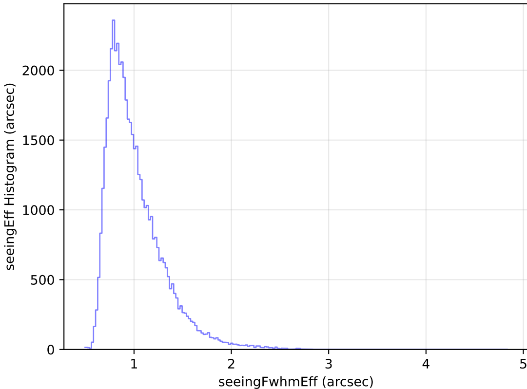
internal_u_expt27_nscale1.1v3.4_10yrs Yr 1 r band: seeingEff Histogram
