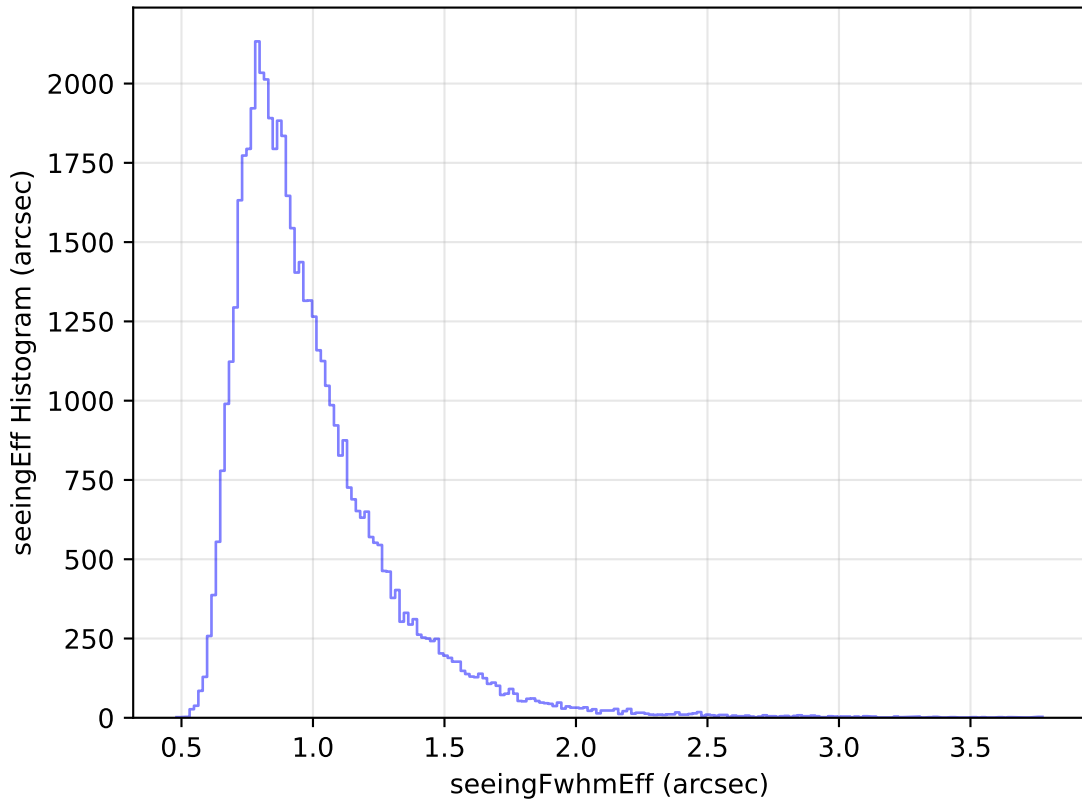
internal_u_expt27_nscale1.1v3.4_10yrs Yr 1 i band: seeingEff Histogram
