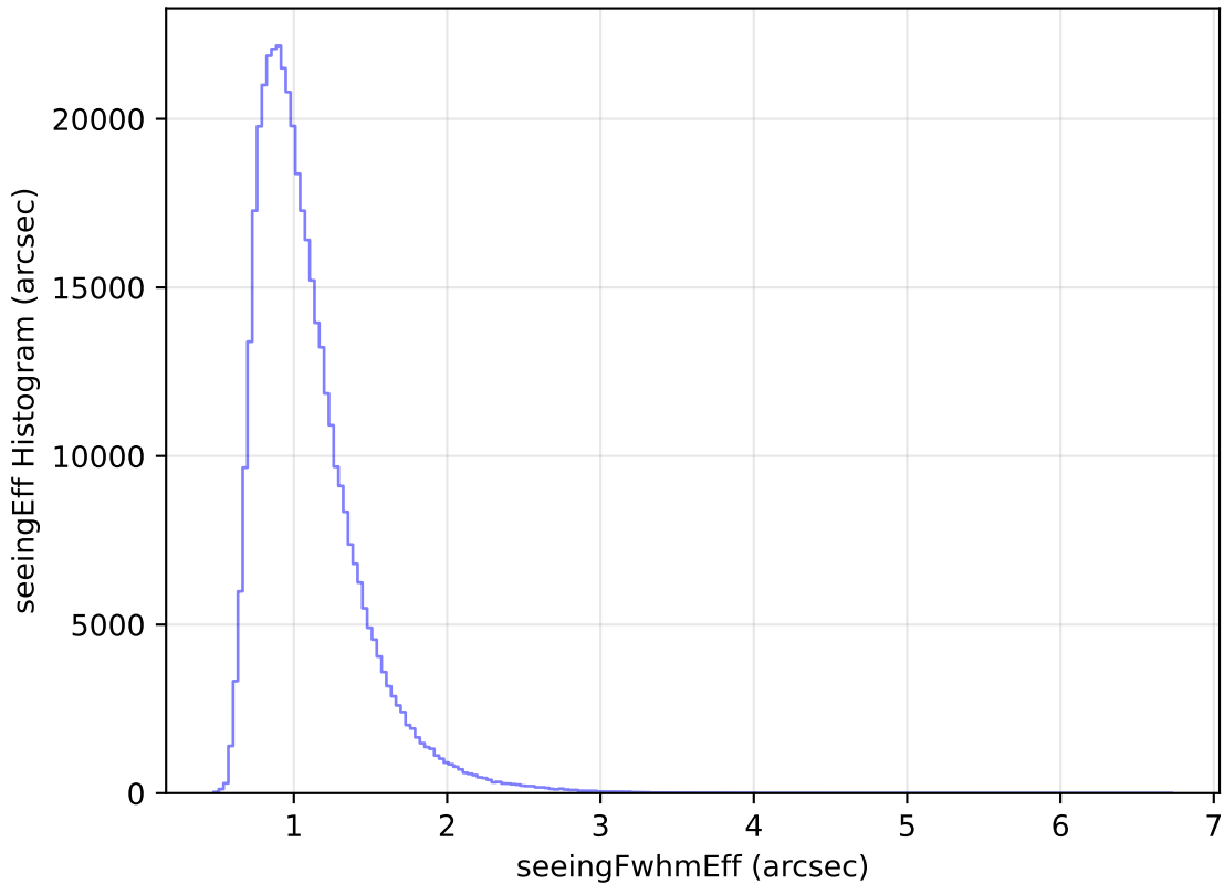
internal_u_expt27_nscale1.1v3.4_10yrs WFD z band: seeingEff Histogram
