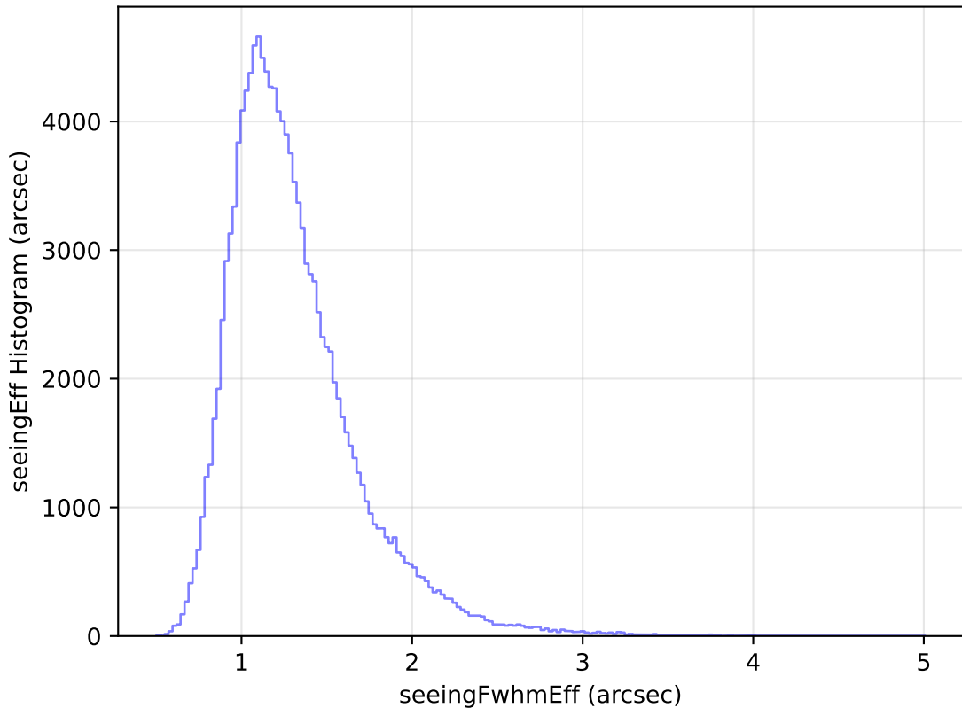
internal_u_expt27_nscale1.1v3.4_10yrs WFD u band: seeingEff Histogram
