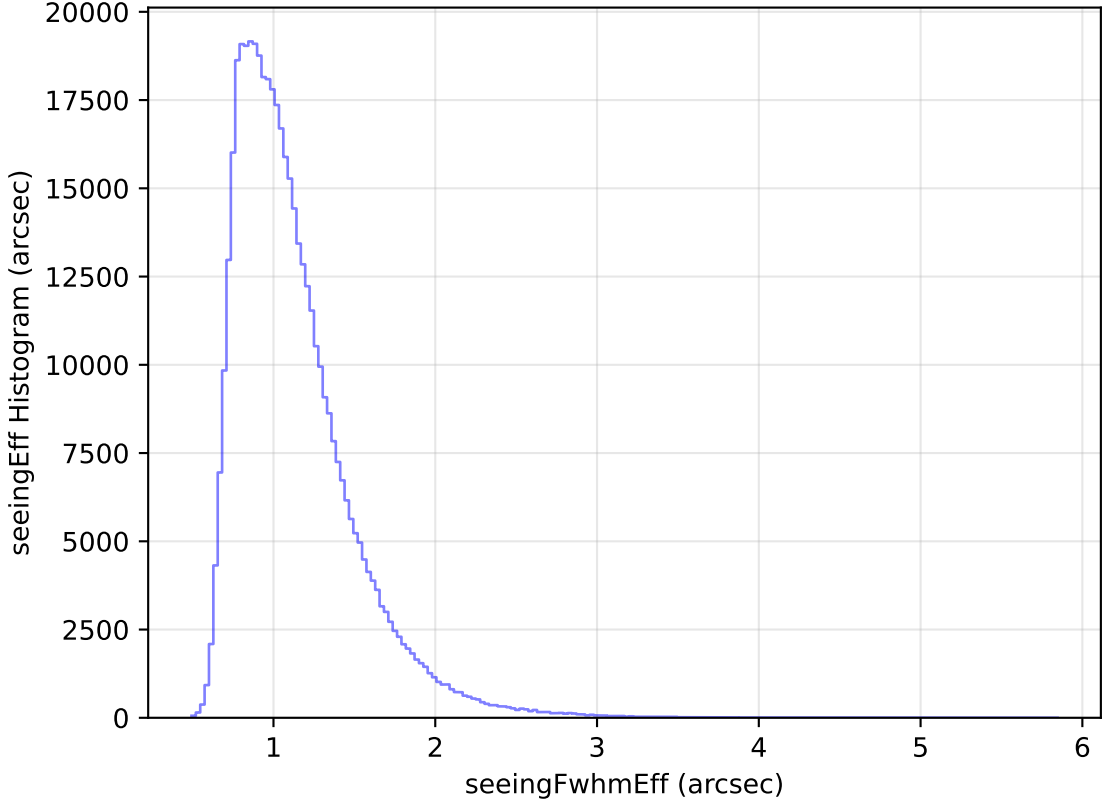
internal_u_expt27_nscale1.1v3.4_10yrs WFD r band: seeingEff Histogram
