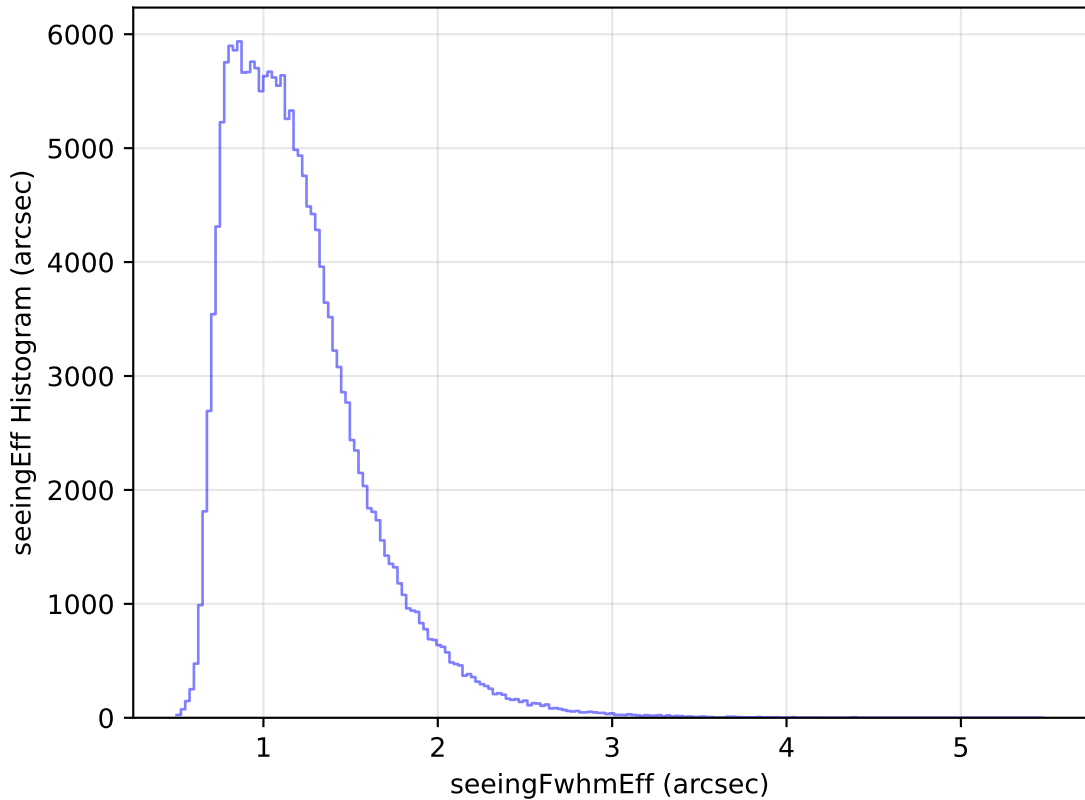
internal_u_expt27_nscale1.1v3.4_10yrs WFD g band: seeingEff Histogram
