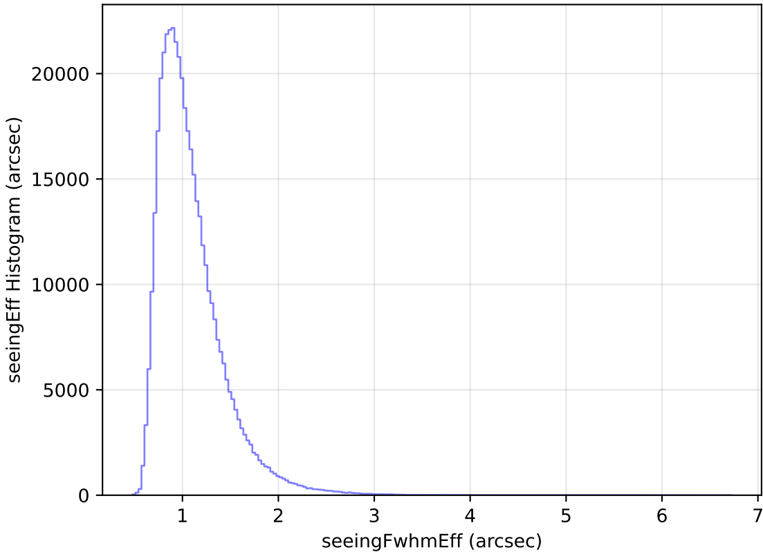
internal_u_expt27_nscale1.1v3.4_10yrs All sky z band: seeingEff Histogram
