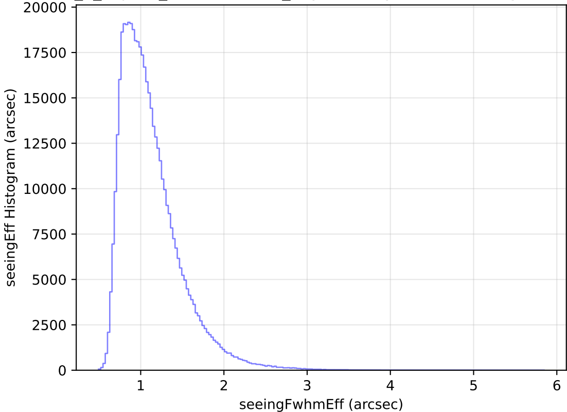
internal_u_expt27_nscale1.1v3.4_10yrs All sky r band: seeingEff Histogram
