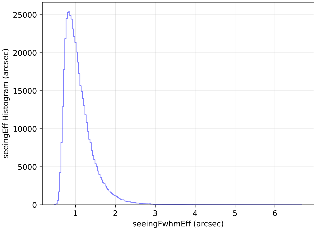
internal_u_expt27_nscale1.1v3.4_10yrs All sky i band: seeingEff Histogram
