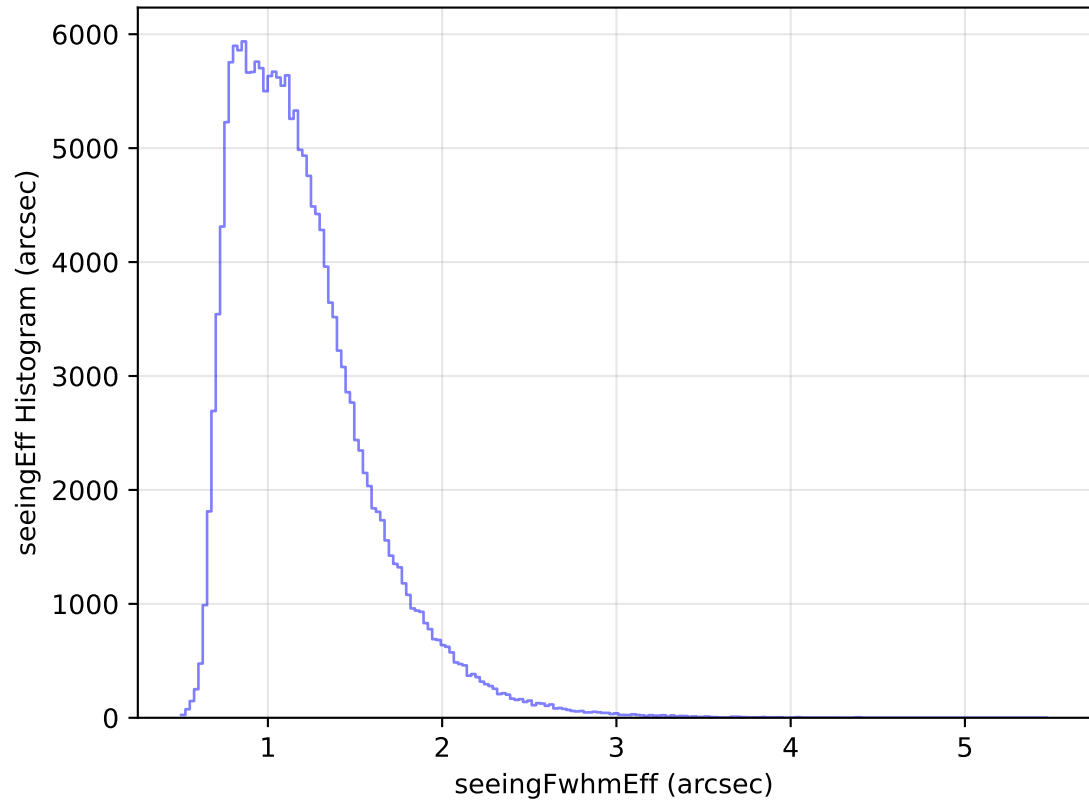
internal_u_expt27_nscale1.1v3.4_10yrs All sky g band: seeingEff Histogram
