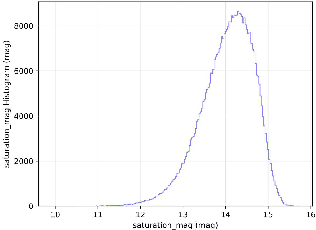
internal_u_expt27_nscale1.1v3.4_10yrs WFD z band: saturation_mag Histogram
