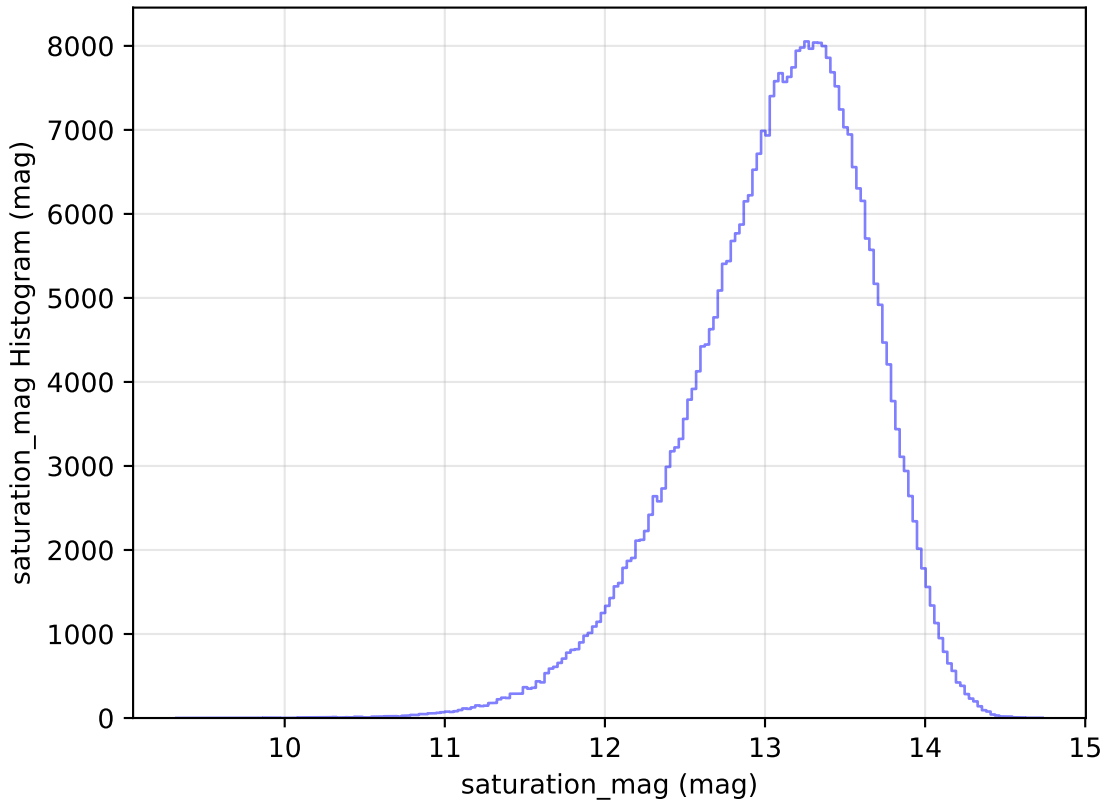
internal_u_expt27_nscale1.1v3.4_10yrs WFD y band: saturation_mag Histogram
