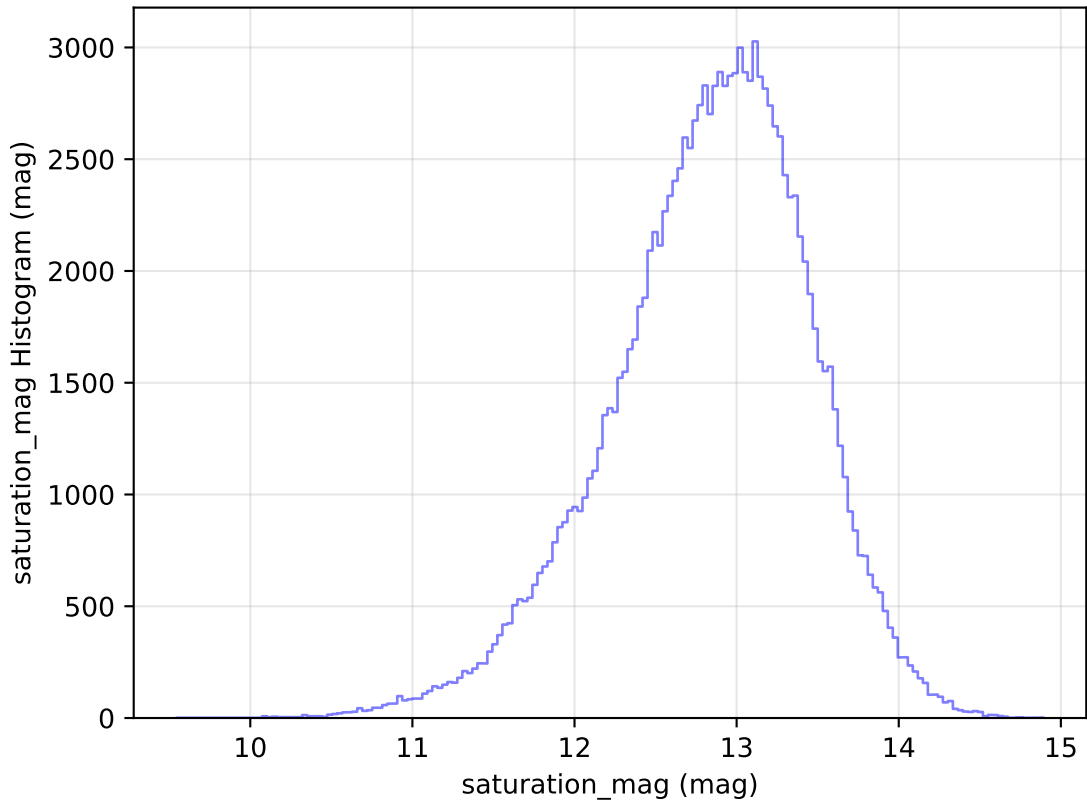
internal_u_expt27_nscale1.1v3.4_10yrs WFD u band: saturation_mag Histogram
