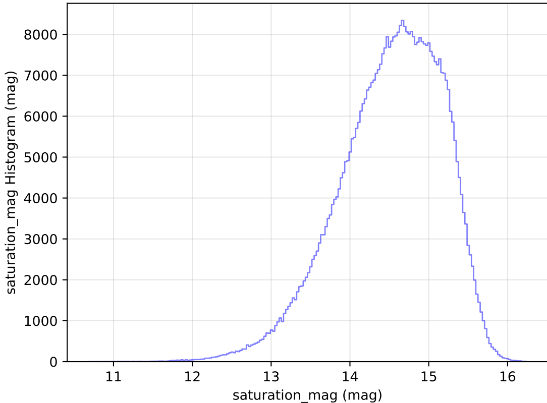
internal_u_expt27_nscale1.1v3.4_10yrs WFD r band: saturation_mag Histogram
