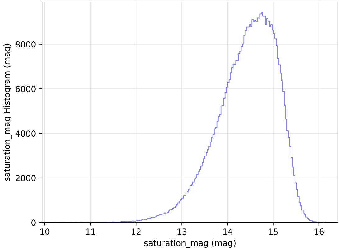
internal_u_expt27_nscale1.1v3.4_10yrs WFD i band: saturation_mag Histogram
