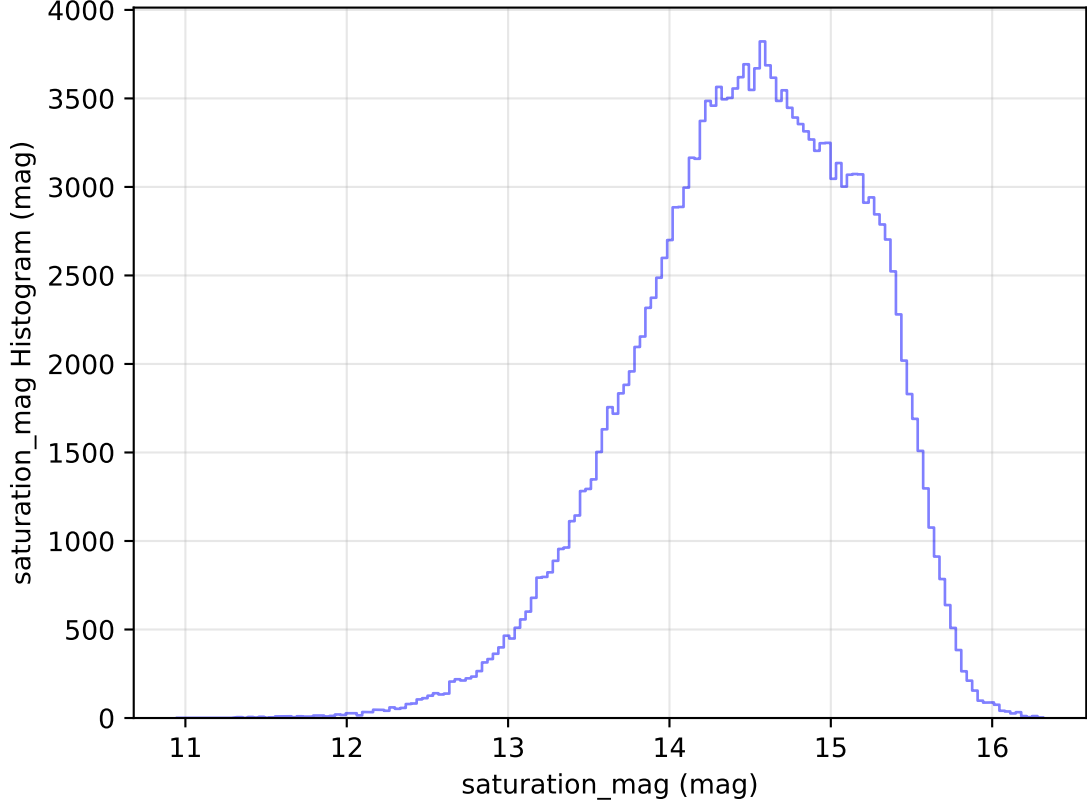
internal_u_expt27_nscale1.1v3.4_10yrs WFD g band: saturation_mag Histogram
