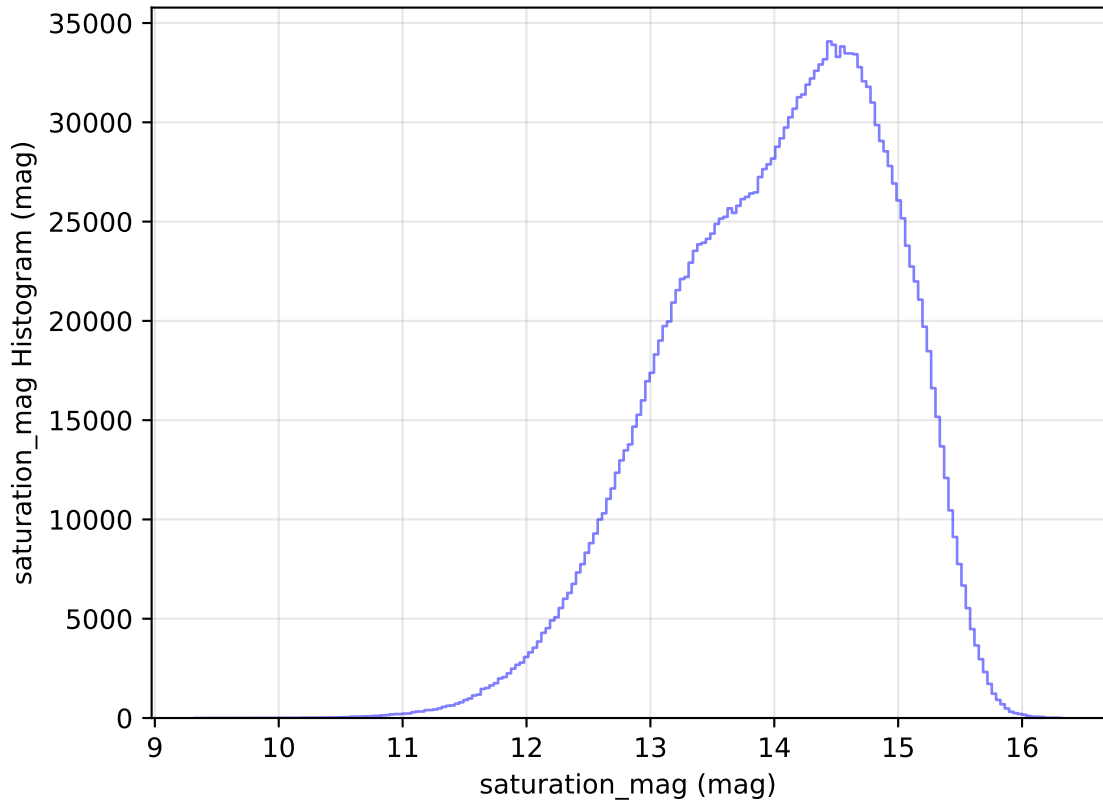
internal_u_expt27_nscale1.1v3.4_10yrs WFD all bands: saturation_mag Histogram
