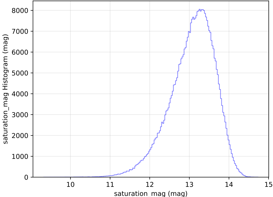
internal_u_expt27_nscale1.1v3.4_10yrs All sky y band: saturation_mag Histogram
