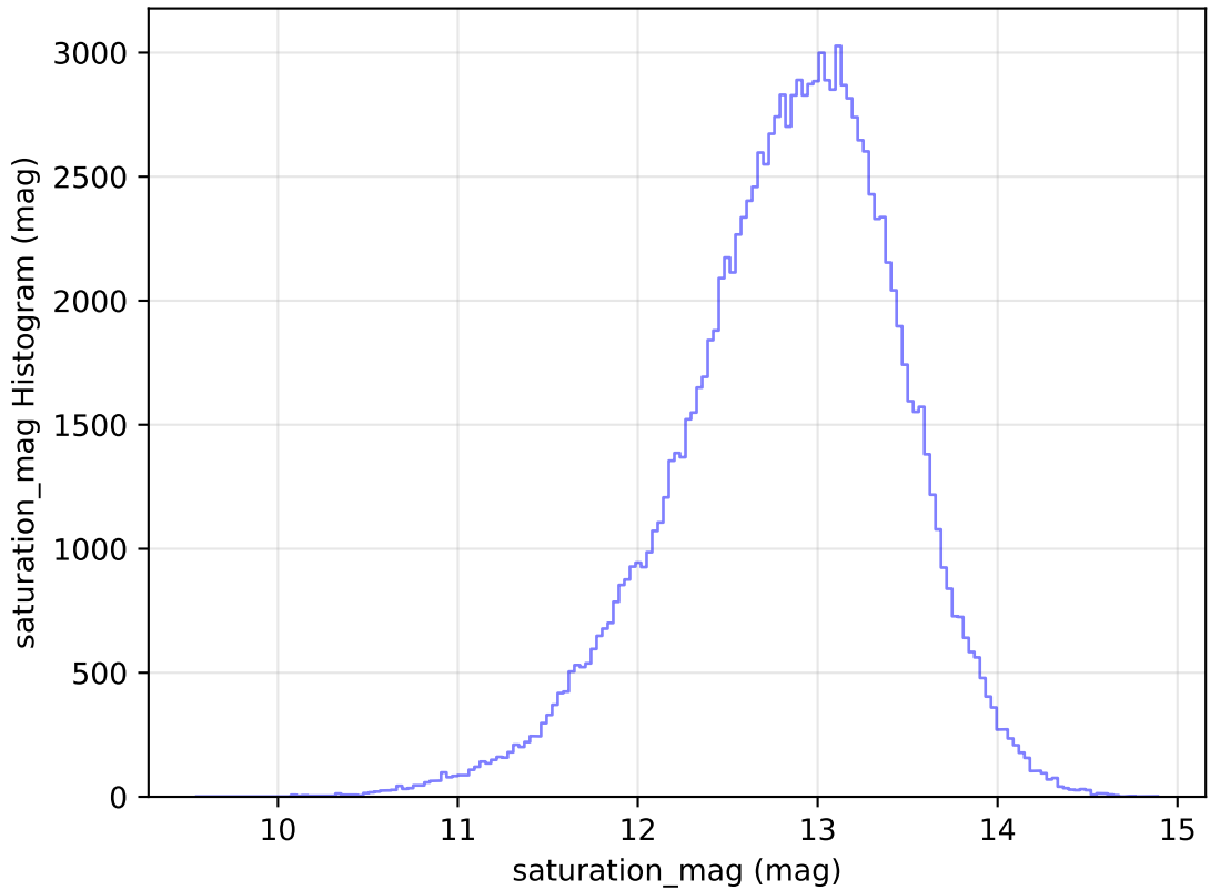
internal_u_expt27_nscale1.1v3.4_10yrs All sky u band: saturation_mag Histogram
