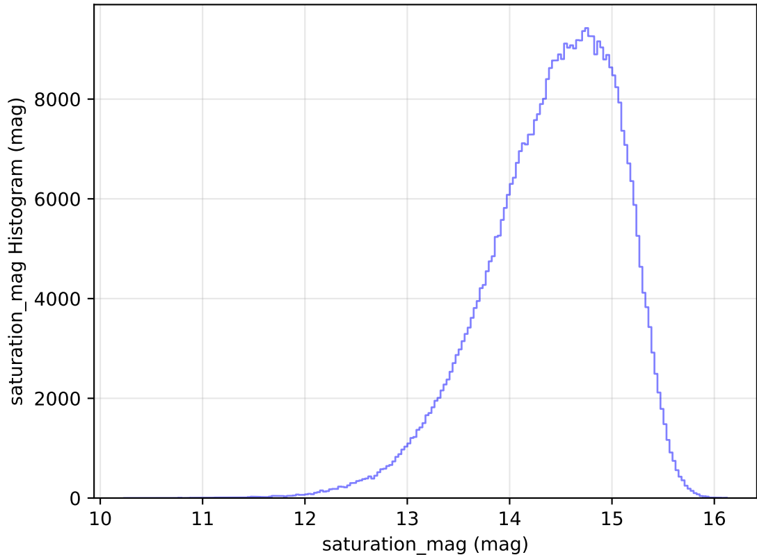
internal_u_expt27_nscale1.1v3.4_10yrs All sky i band: saturation_mag Histogram
