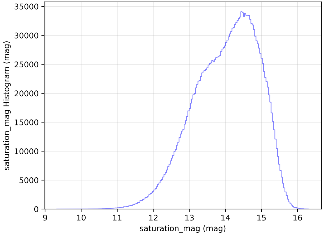
internal_u_expt27_nscale1.1v3.4_10yrs All sky all bands: saturation_mag Histogram
