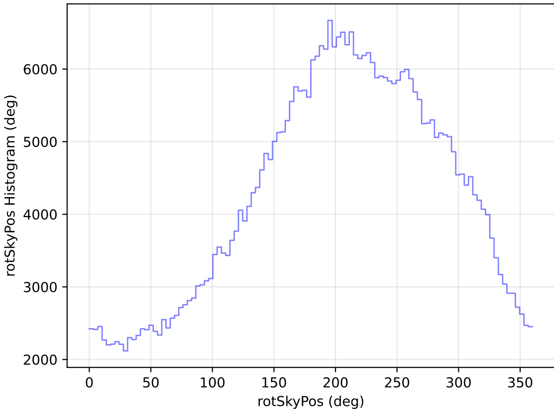
internal_u_expt27_nscale1.1v3.4_10yrs WFD z band: rotSkyPos Histogram
