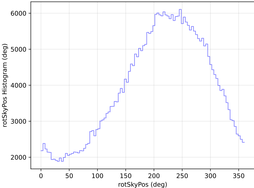
internal_u_expt27_nscale1.1v3.4_10yrs WFD y band: rotSkyPos Histogram
