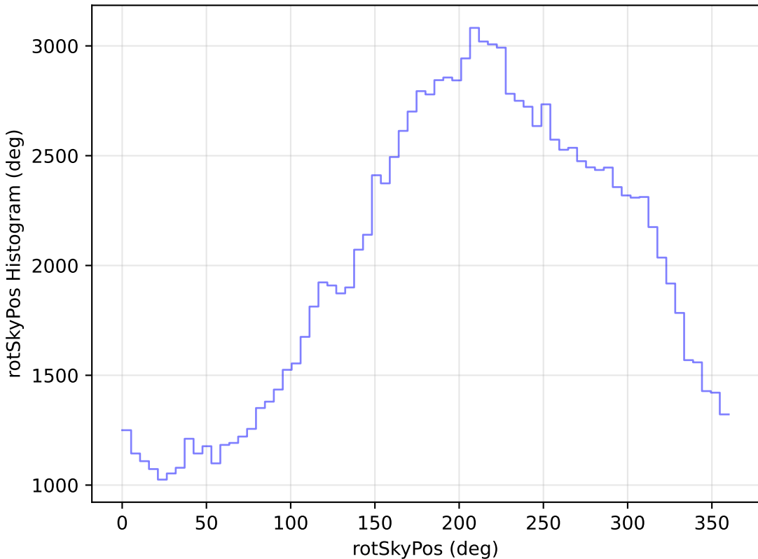
internal_u_expt27_nscale1.1v3.4_10yrs WFD u band: rotSkyPos Histogram
