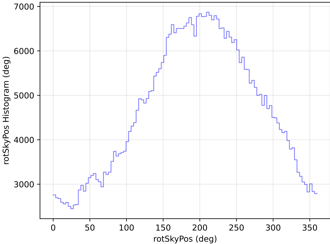
internal_u_expt27_nscale1.1v3.4_10yrs WFD r band: rotSkyPos Histogram
