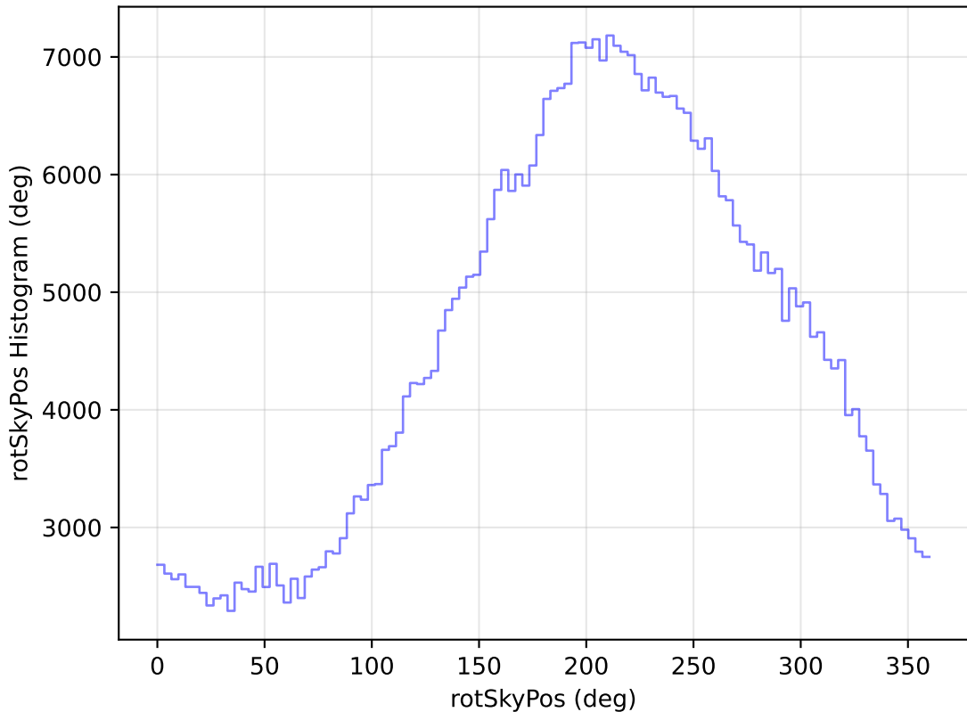
internal_u_expt27_nscale1.1v3.4_10yrs WFD i band: rotSkyPos Histogram
