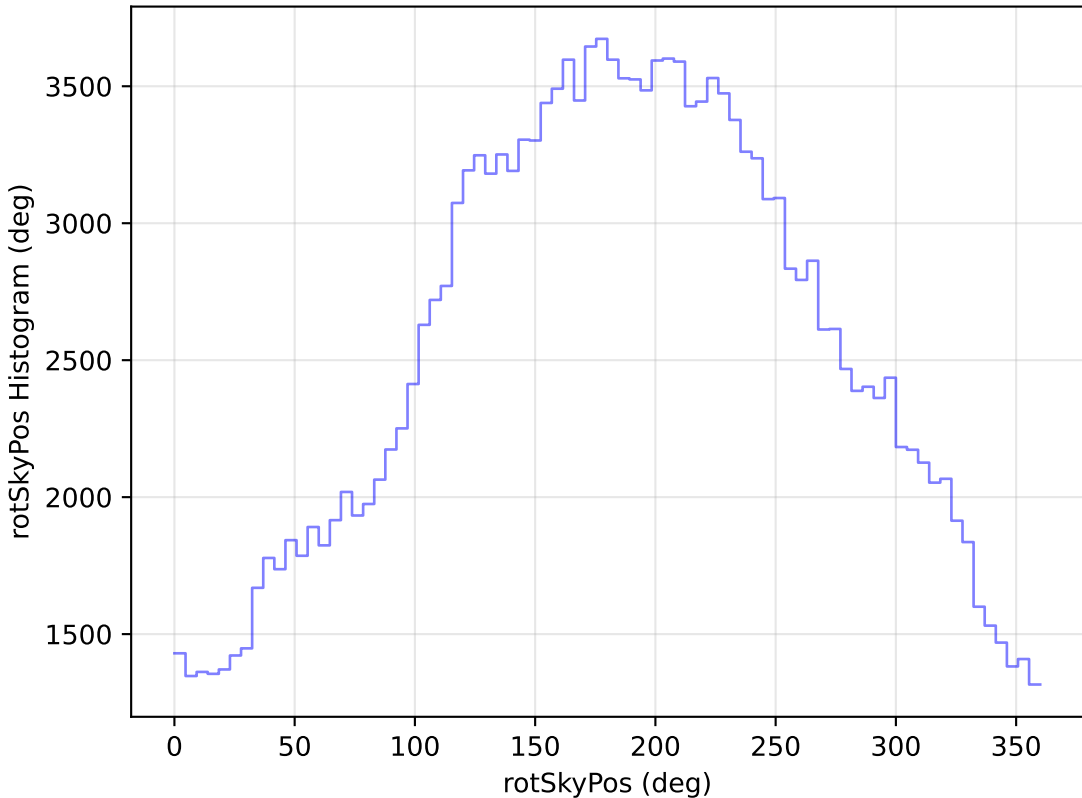
internal_u_expt27_nscale1.1v3.4_10yrs WFD g band: rotSkyPos Histogram
