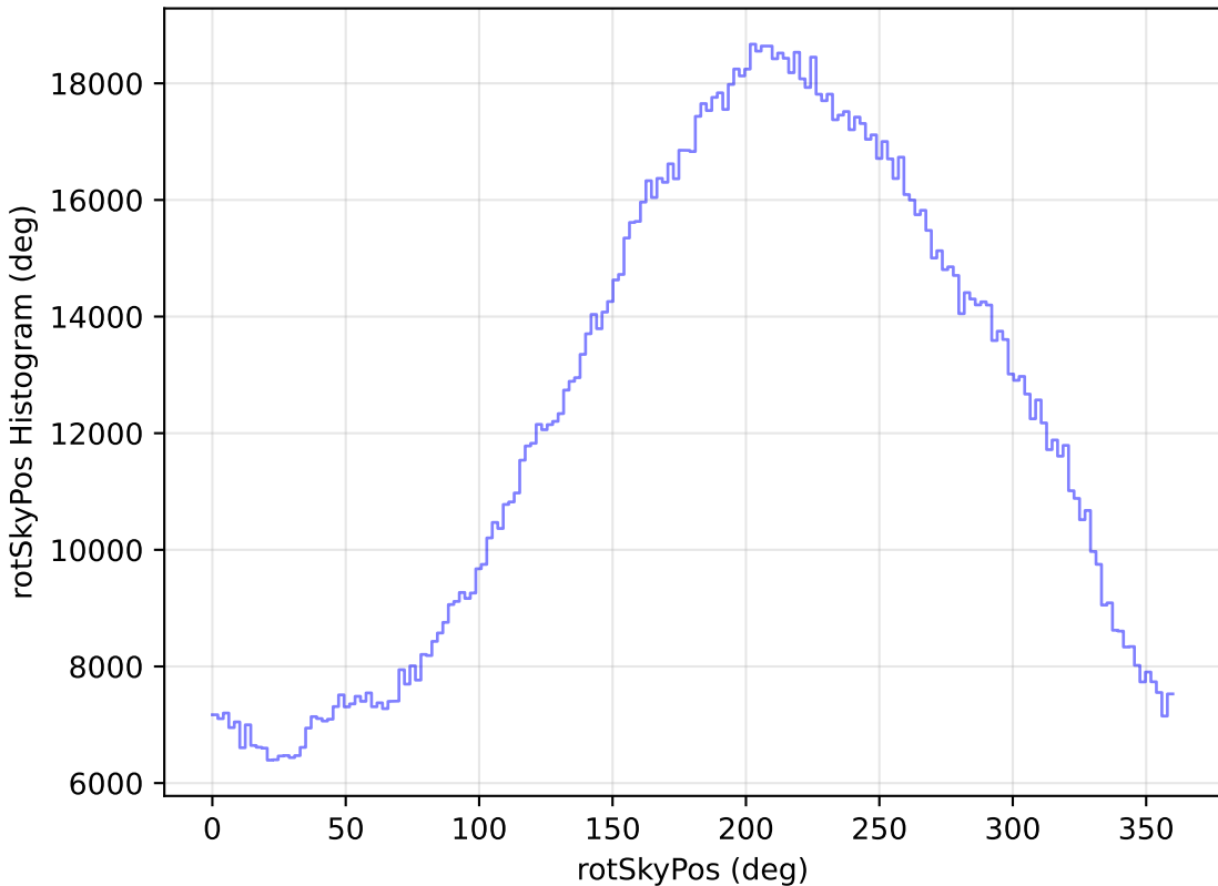
internal_u_expt27_nscale1.1v3.4_10yrs WFD all bands: rotSkyPos Histogram
