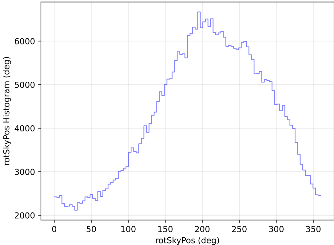
internal_u_expt27_nscale1.1v3.4_10yrs All sky z band: rotSkyPos Histogram
