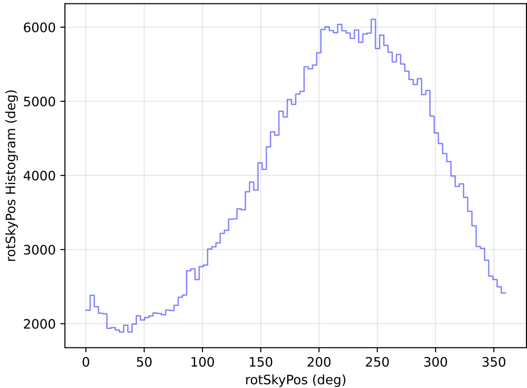
internal_u_expt27_nscale1.1v3.4_10yrs All sky y band: rotSkyPos Histogram
