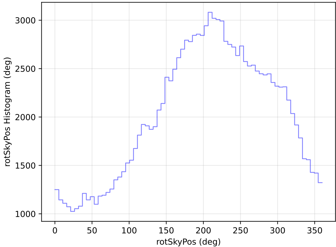
internal_u_expt27_nscale1.1v3.4_10yrs All sky u band: rotSkyPos Histogram
