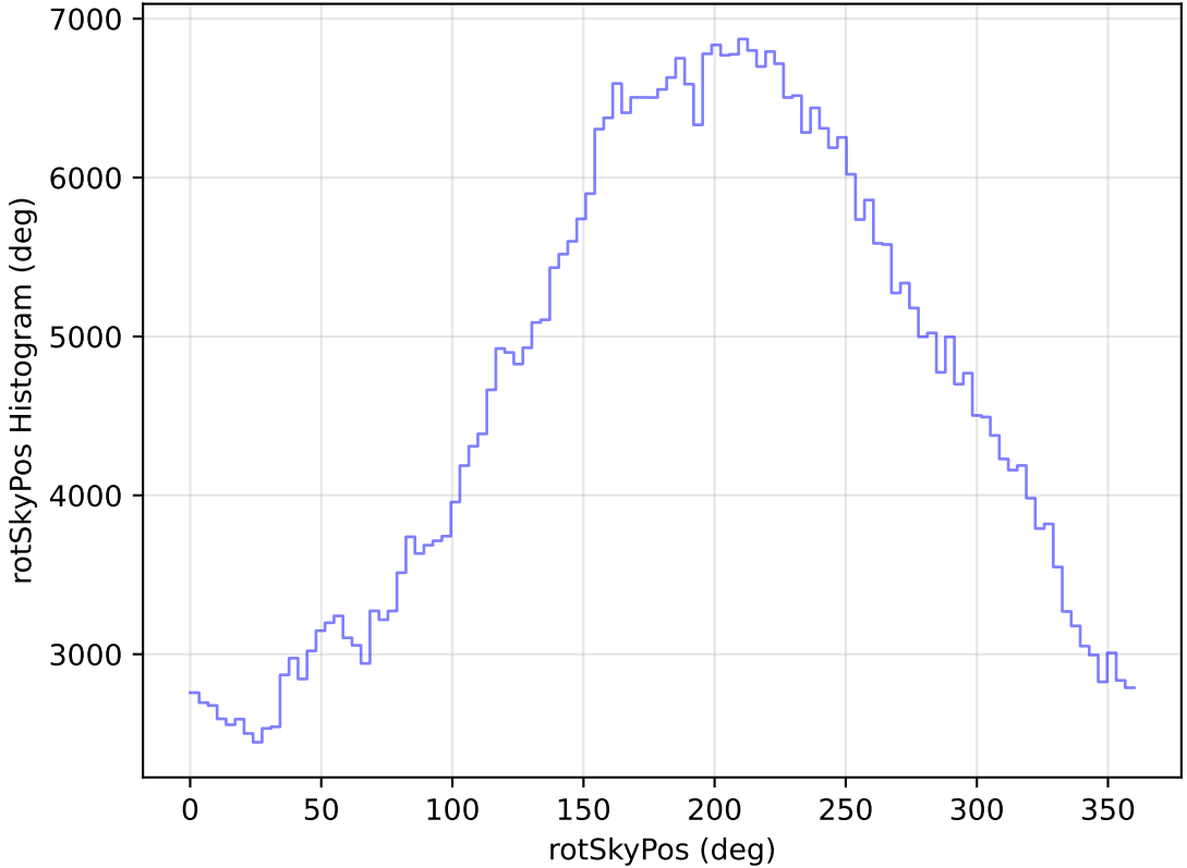
internal_u_expt27_nscale1.1v3.4_10yrs All sky r band: rotSkyPos Histogram
