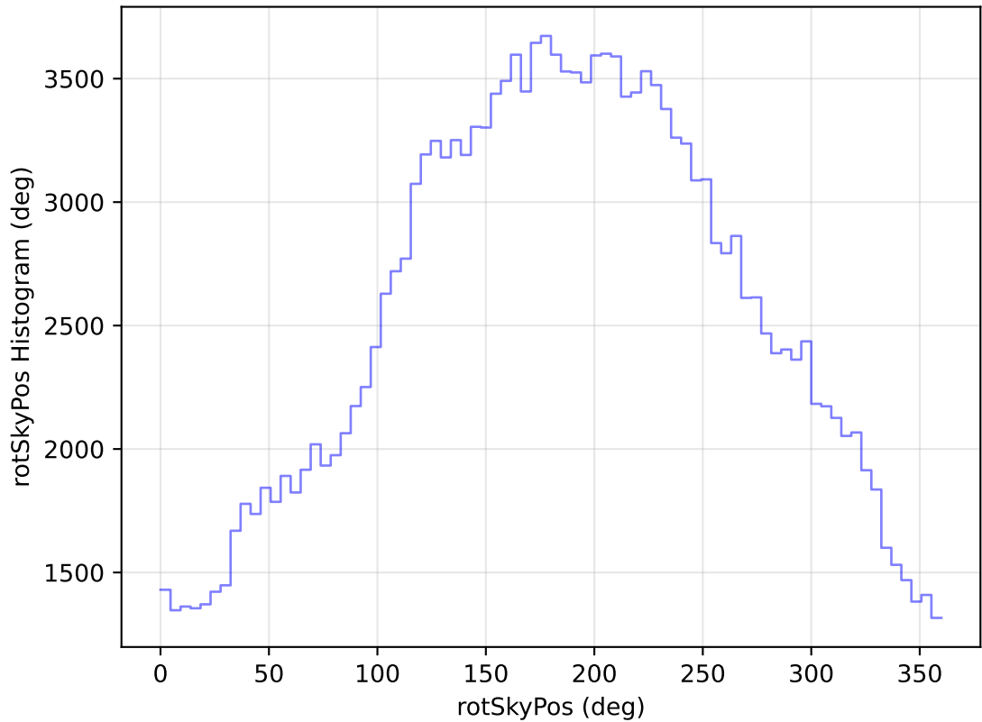
internal_u_expt27_nscale1.1v3.4_10yrs All sky g band: rotSkyPos Histogram
