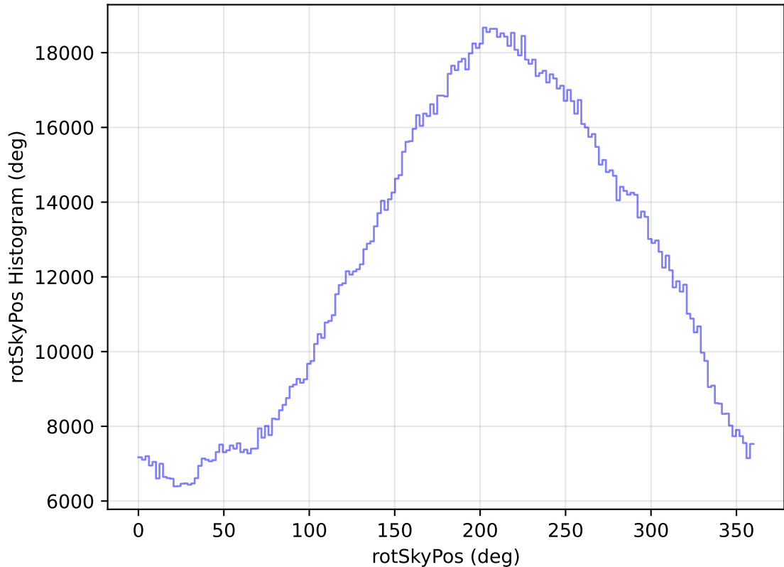
internal_u_expt27_nscale1.1v3.4_10yrs All sky all bands: rotSkyPos Histogram
