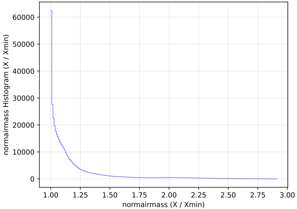
internal_u_expt27_nscale1.1v3.4_10yrs WFD z band: normairmass Histogram
