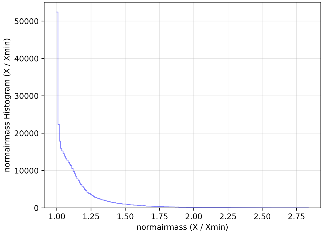
internal_u_expt27_nscale1.1v3.4_10yrs WFD y band: normairmass Histogram
