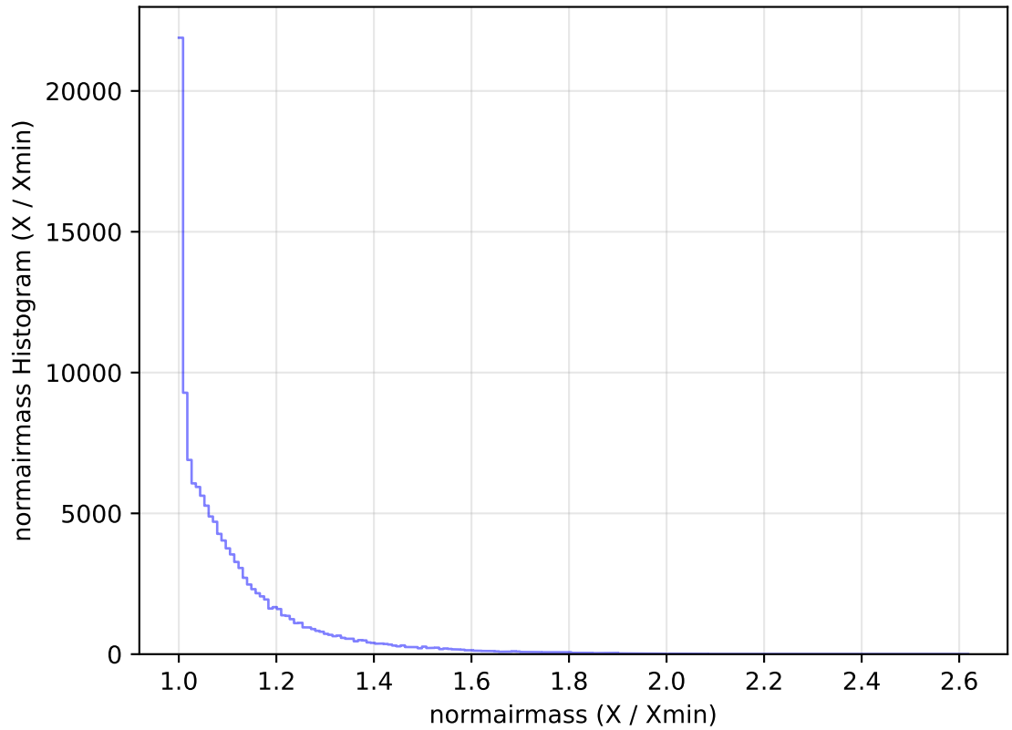
internal_u_expt27_nscale1.1v3.4_10yrs WFD u band: normairmass Histogram
