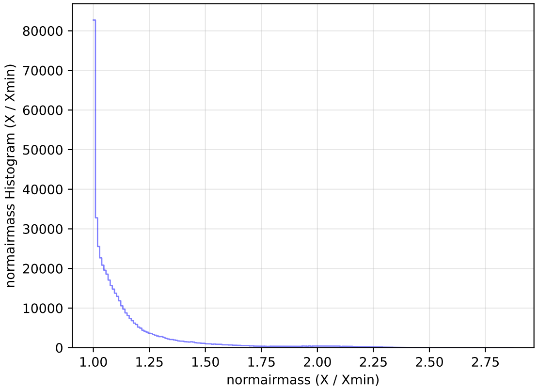
internal_u_expt27_nscale1.1v3.4_10yrs WFD r band: normairmass Histogram
