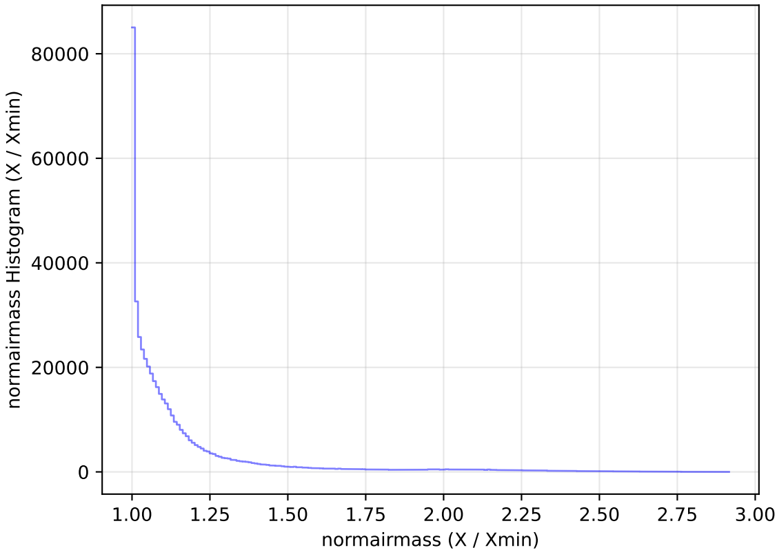
internal_u_expt27_nscale1.1v3.4_10yrs WFD i band: normairmass Histogram
