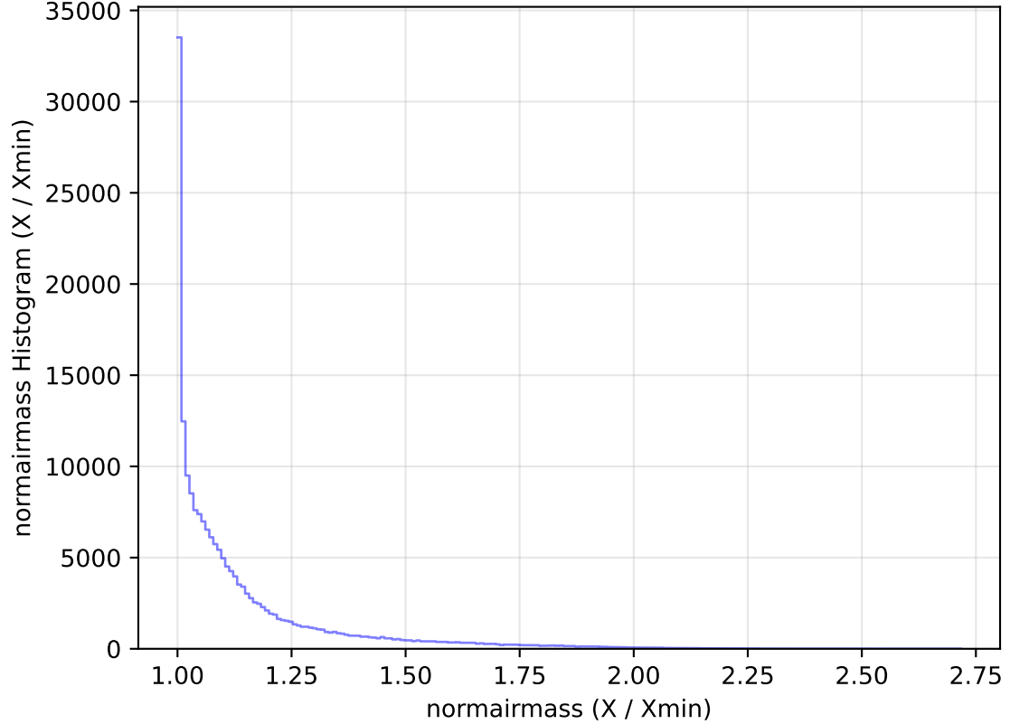
internal_u_expt27_nscale1.1v3.4_10yrs WFD g band: normairmass Histogram
