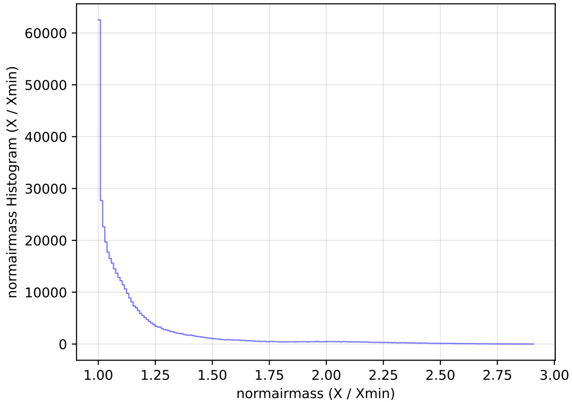
internal_u_expt27_nscale1.1v3.4_10yrs All sky z band: normairmass Histogram
